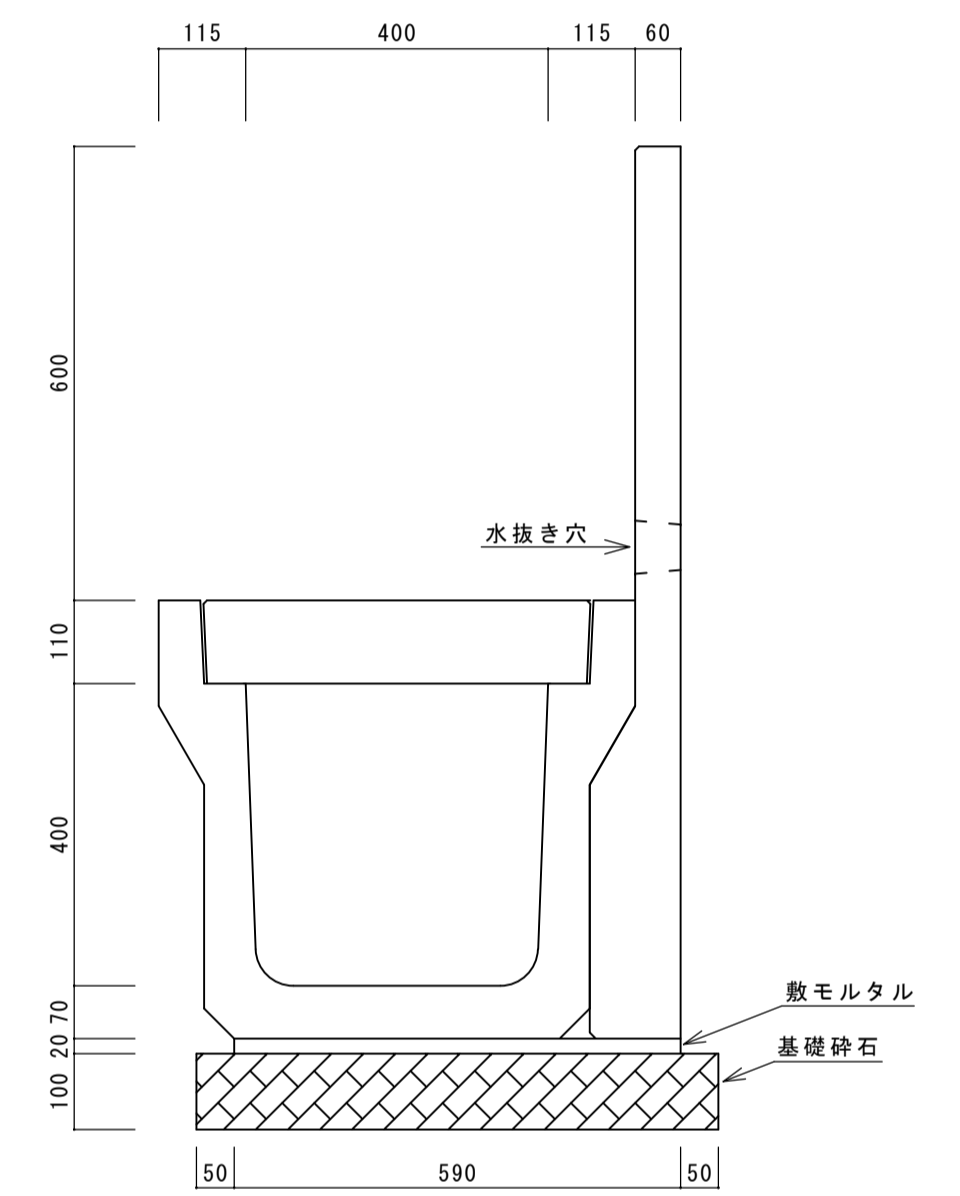
U h 柵3種400A-6 S=1/10
